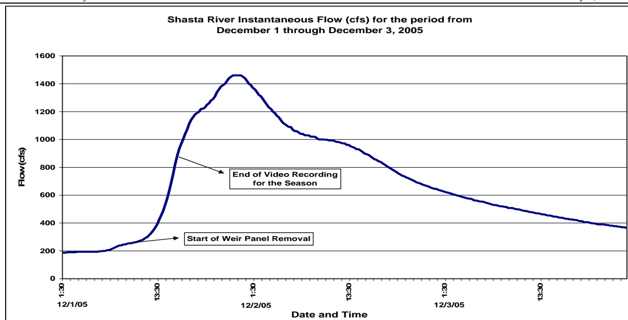
Figure 2. Shasta River flows (cfs) recorded at the USGS Gauge #11517500 from December 1 through December 3, 2005.
